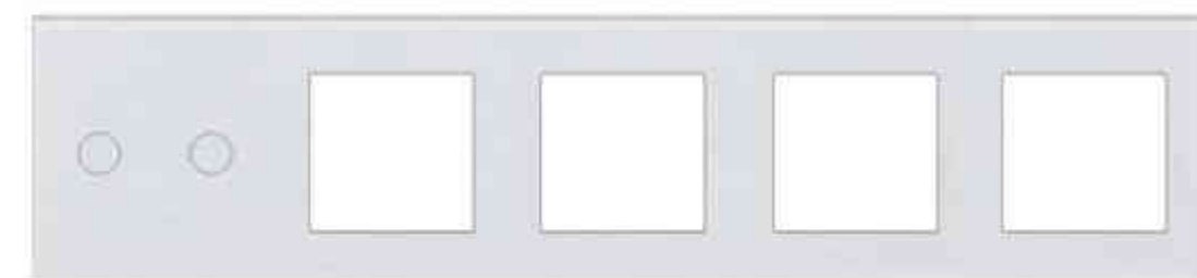
1g+4fold 86*370mm GP037 2g+4fold 86*370mm GP038 3g+4fold 86*370mm GP039
