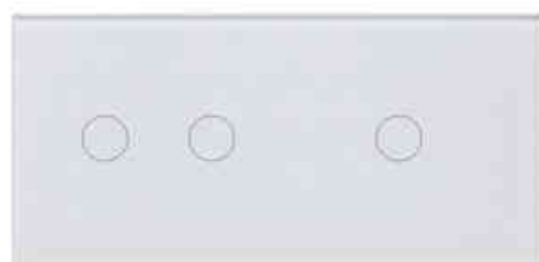
2g+1g GLS Panel 86*157mm GP014 86*146mm GP014UK
